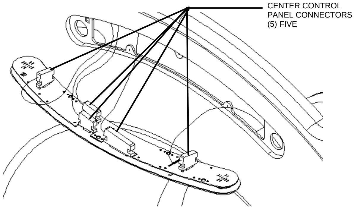
CENTER CONTROL PANEL DETAIL ILLUSTRATION 1-2
