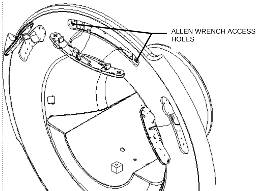
CONTROL PANEL LOCATIONS ILLUSTRATION 1-1
